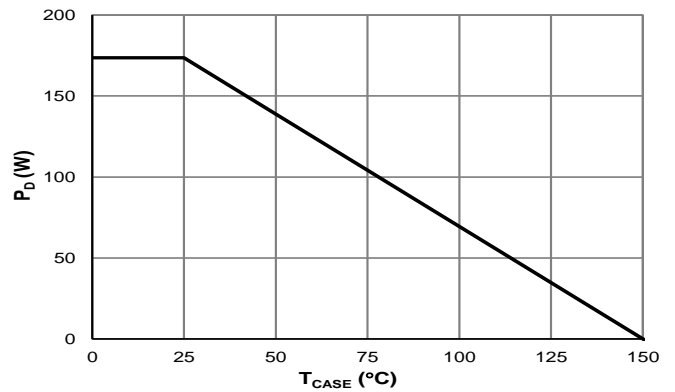
Figure 10: Power De-rating
