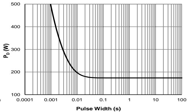
Figure 12: Single Pulse Power Rating, Junction-to-Case
