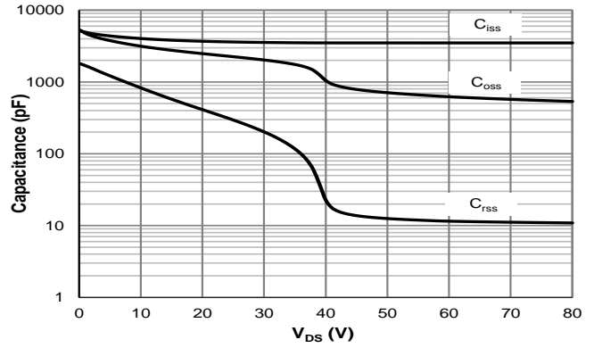
Figure 8: Capacitance Characteristics
