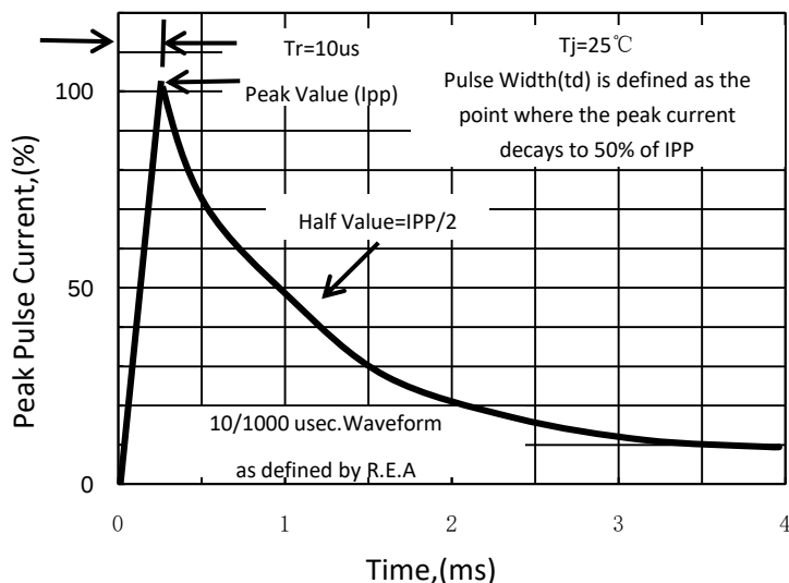
Fig. 5-Pulse Waveform
