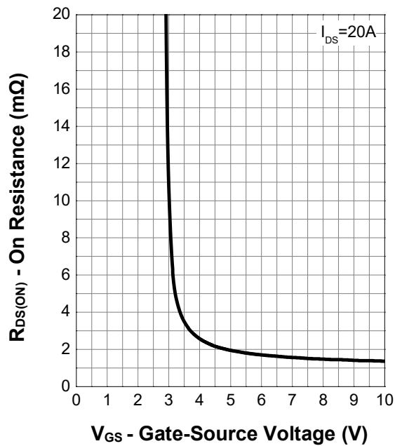
Transfer Characteristics
