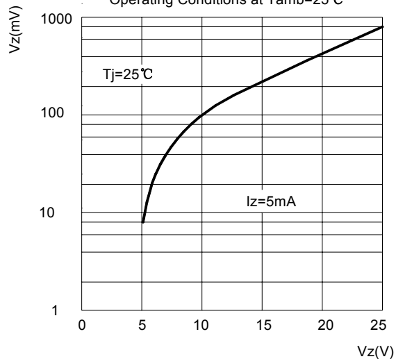
FIG2: Typical Change of Working Voltage under Operating Conditions at T_{amb}=25^{\circ}C
