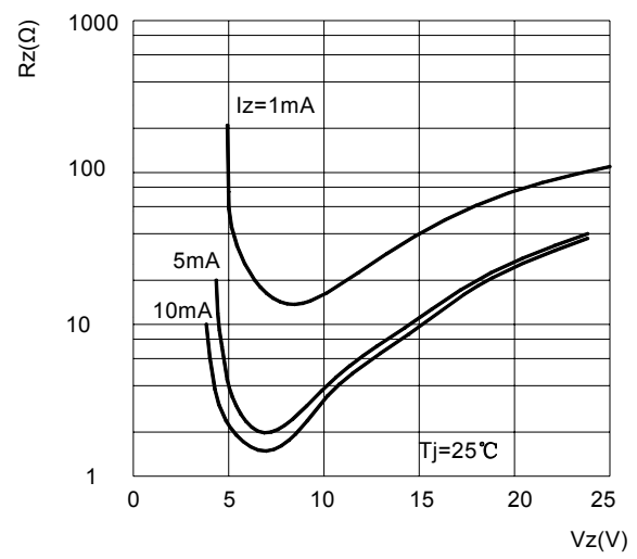
FIG8: Differential Z-Resistance vs. Z-Voltage
