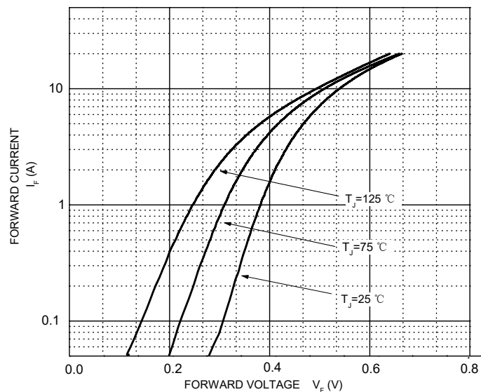
Forward Characteristics
