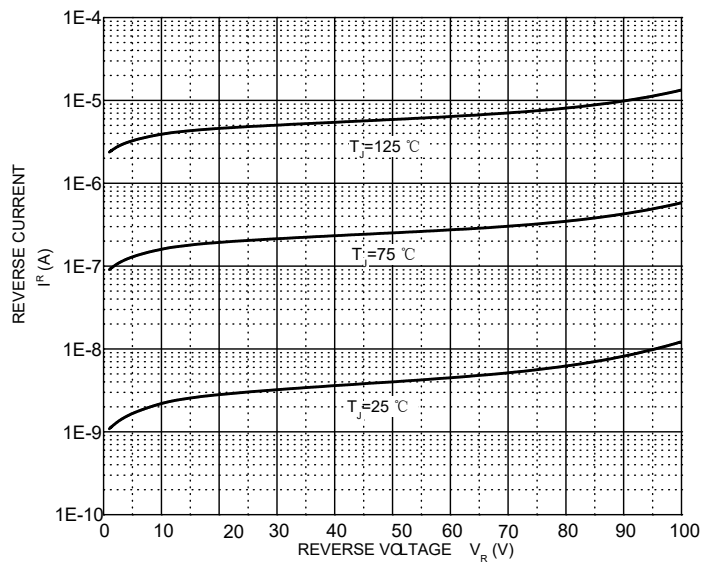
Reverse Characteristics
