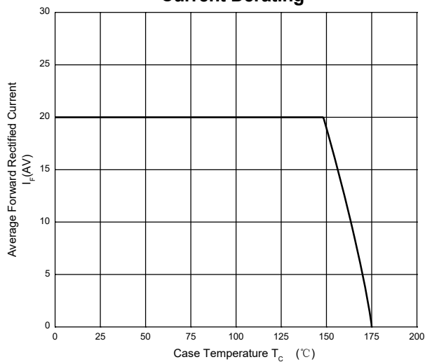
Current Derating
