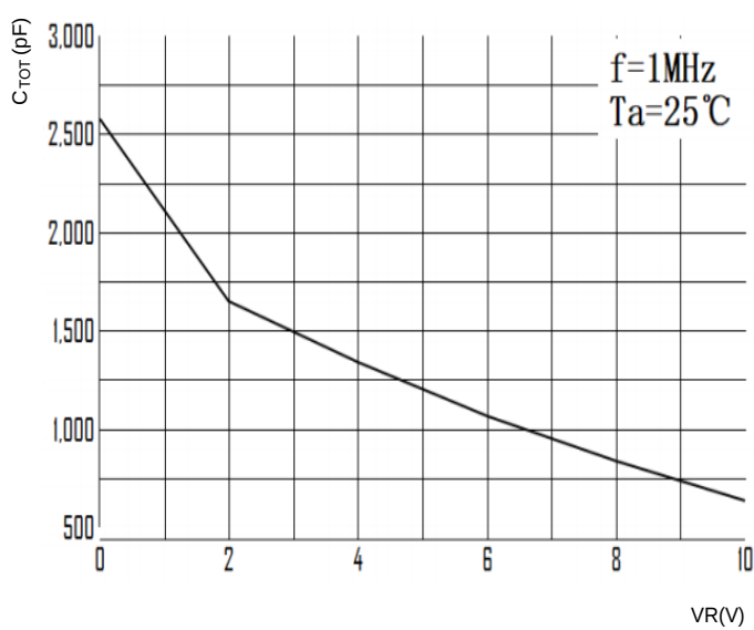
FIG.3: TOTAL CAPACITANCE DERATING CURVE
