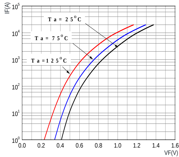
FIG1: Instantaneous Forward Voltage
