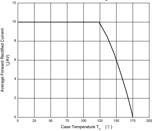
Current Derating
