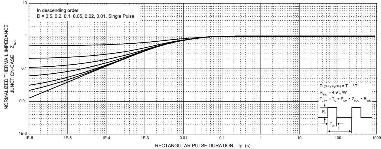
MURF10H20CT Transient Thermal Impedance, Junction-Case
