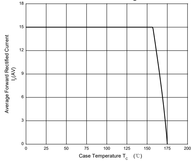
Current Derating
