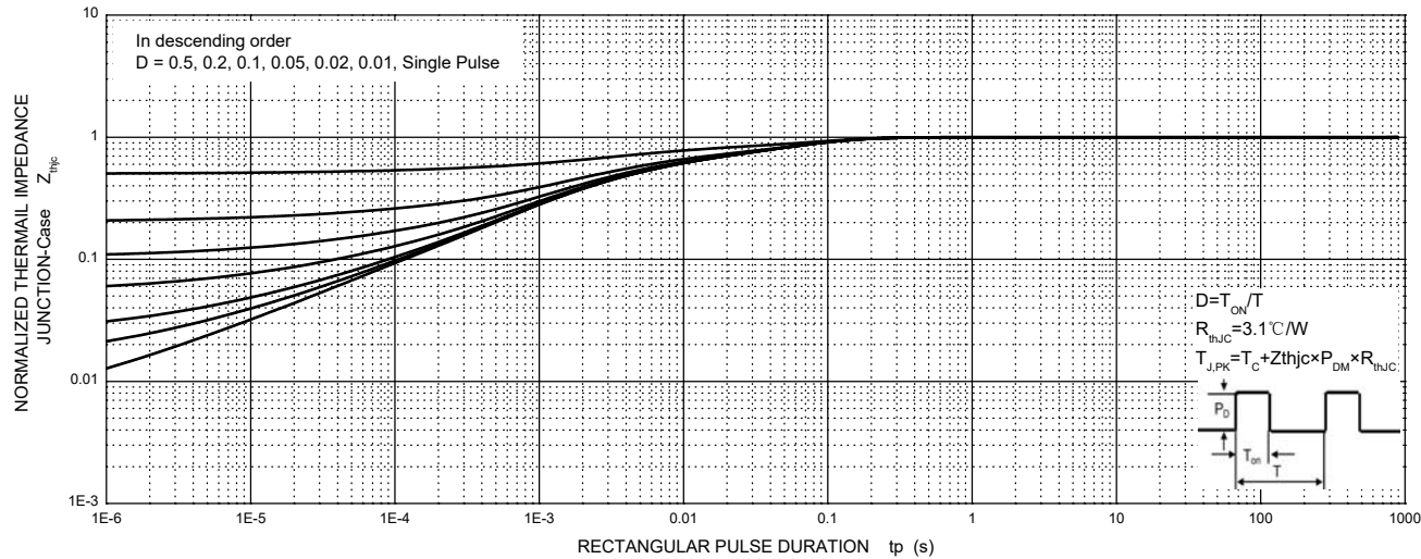
MUR20H40CTB Transient Thermal Impedance, Junction-Case
