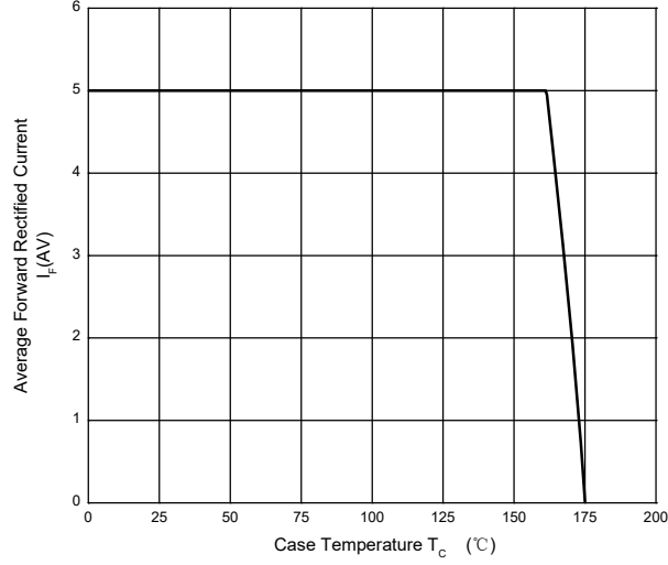
Current Derating
