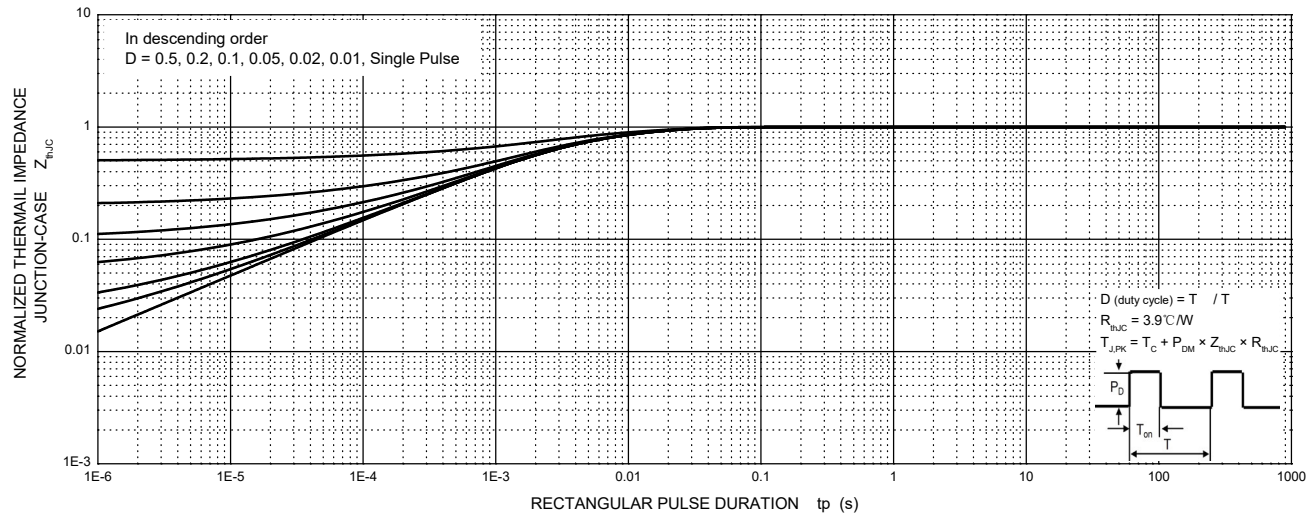
MUR10H20CT Transient Thermal Impedance, Junction-Case
