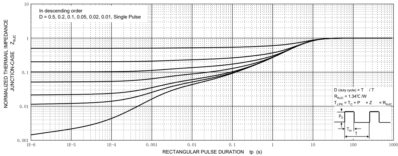
MUR30H60L Transient Thermal Impedance, Junction-Case
