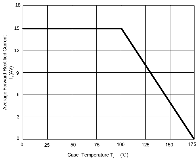
Current Derating
