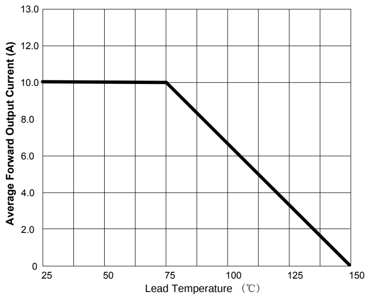
FIG.1: I_o -TL Curve
