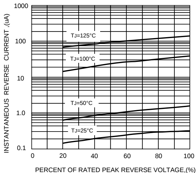
FIG.3-TYPICAL REVERSE CHARACTERISTICS
