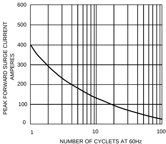
FIG.2-MAXIMUM FORWARD SURGE CURRENT
