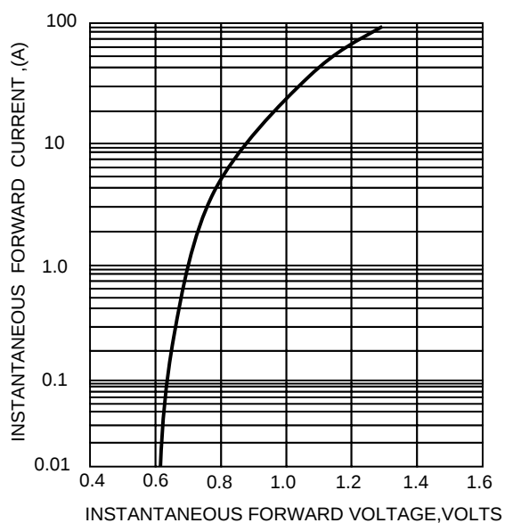
FIG.4-TYPICAL FORWARD CHARACTERISTICS
