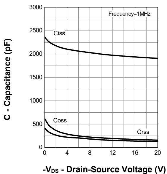
Capacitance
