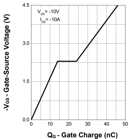
Gate Charge
