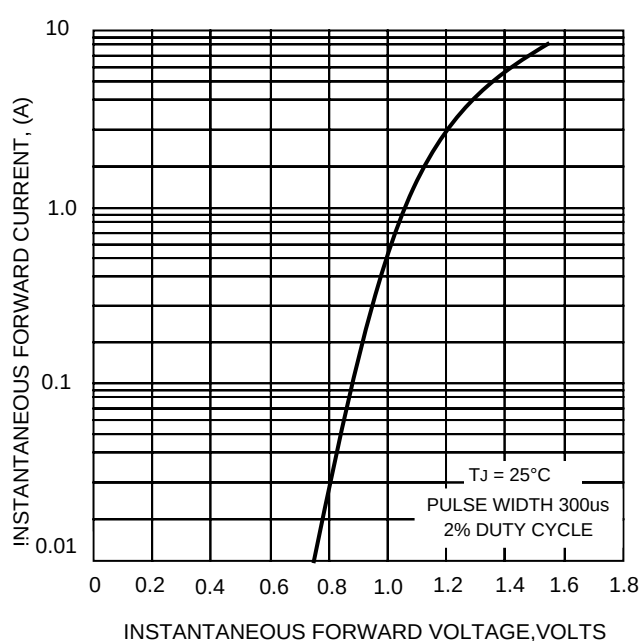
FIG.4-TYPICAL FORWARD CHARACTERISTICS
