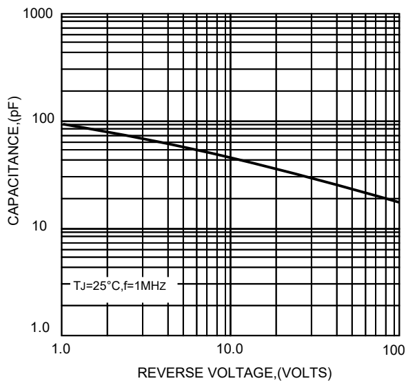
FIG.3-TYPICAL JUNCTION CAPACITANCE
