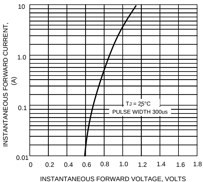
FIG.4-TYPICAL FORWARD CHARACTERISTICS
