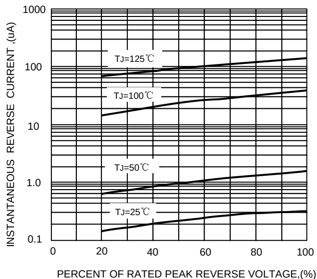
FIG.5-TYPICAL REVERSE CHARACTERISTICS
